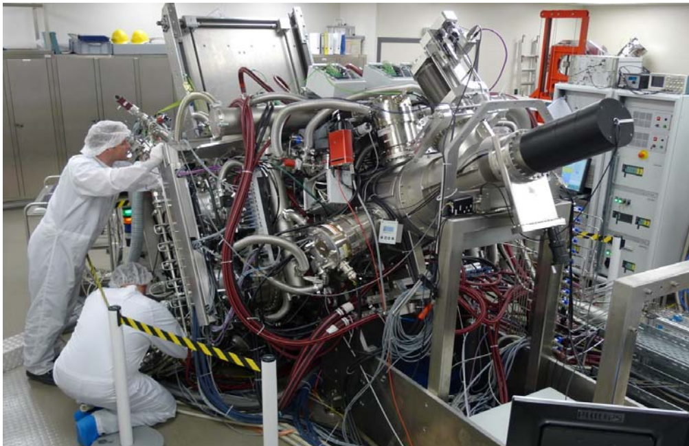
figure 5 Source Collector Module for the NXE 3100
