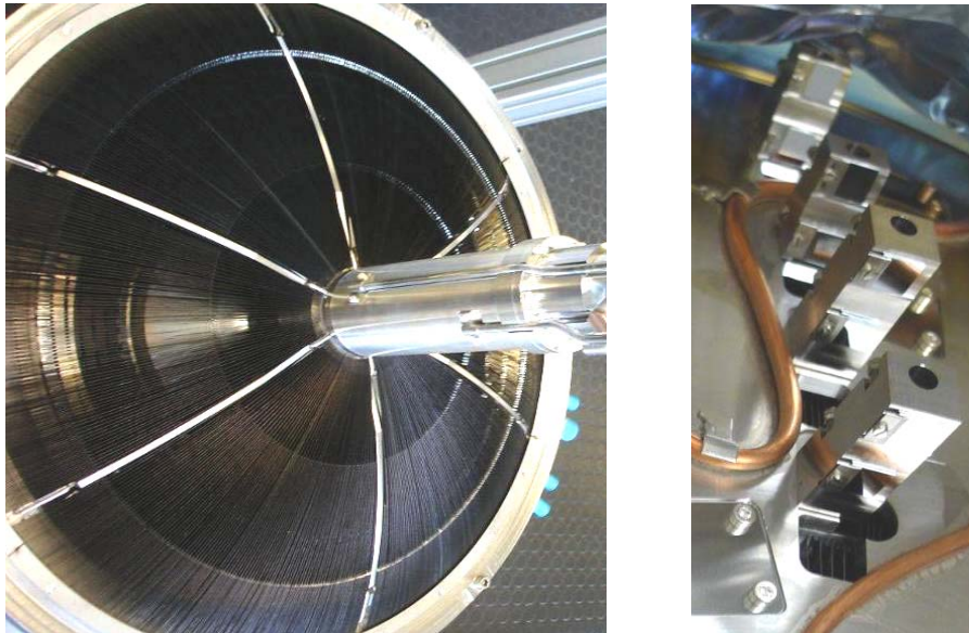
figure 17 Foiltrap from the collector side (left) and arrangement of the collector samples during the longterm tests (right).
