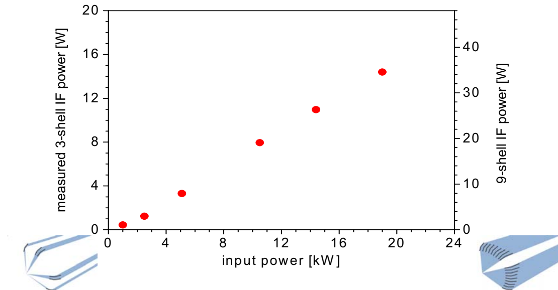
figure 9 EUV power in the intermediate focus in dependence on the electrical input power measured for the 3-shell collector (left y-axis) and extrapolated for the full 9-shell collector (right y-axis)
