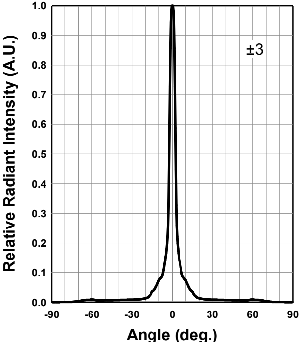
Radiation Characteristics
