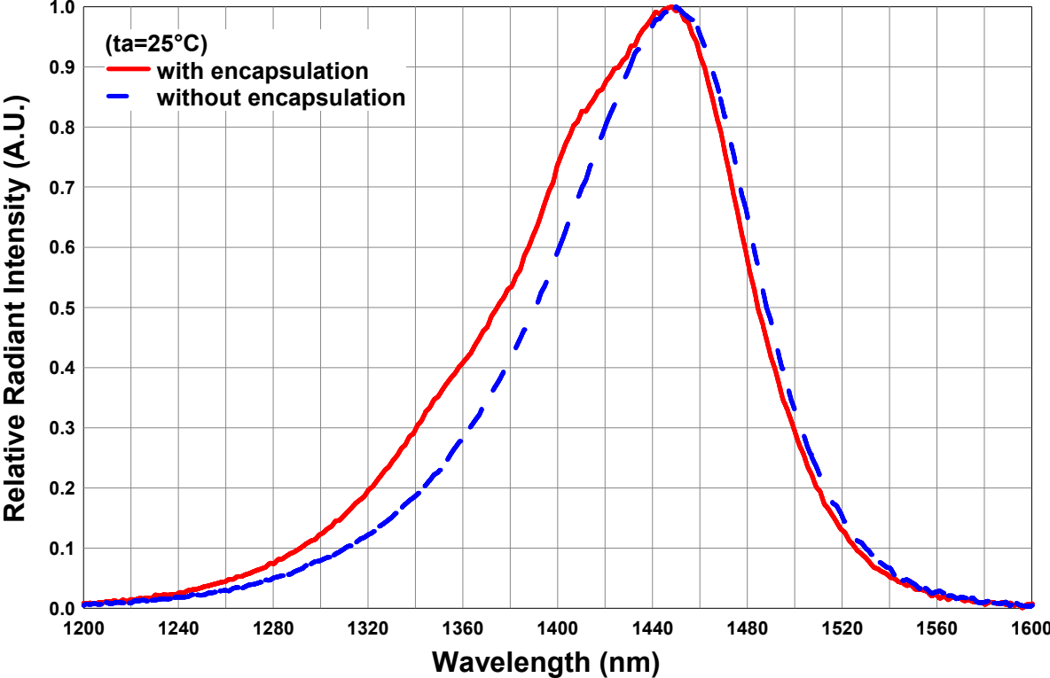
Relative Spectral Emission
