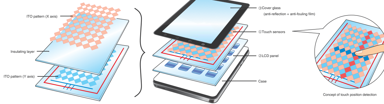
The structure of touch panels
